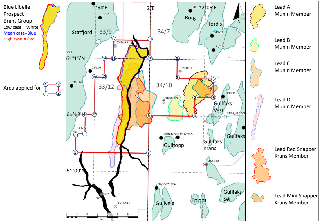
Fig. 4.1 Application area applied for and prospectivity
