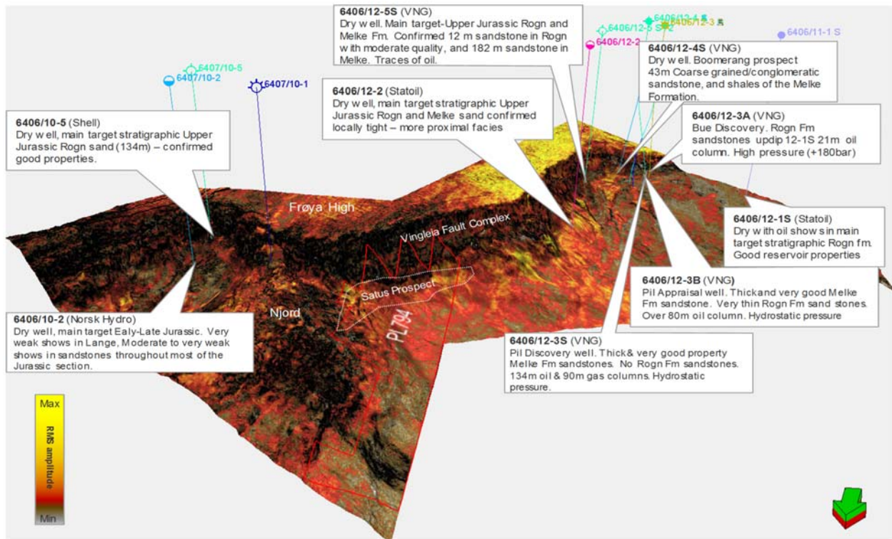
Figure 2a. Oblique view on the hanging wall of the Vingloia Fault Complex. RMS amplitude map of Base Cretaceous Unconformity, PL 794 limits and Satus prospect, and analogue wells in the hanging wall with Late Jurassic targets.
