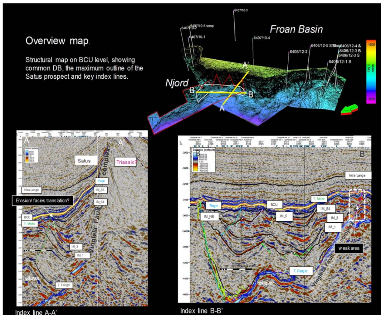
Figure 3. Oblique view to the hanging wall of the Vingleia Fault Complex (VFC) presented in the upper image (Structural time map of the BCU) and depositional concept for PL794 presented in dip (A-A') and strike (B-B') index lines; shown also VFC and local rollover structure controlling geometry of the Late Jurassic sediment deposits in the Satus prospect.
